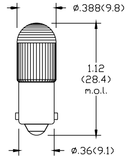
1835LS/1819LS2 Series for GE ET-16
