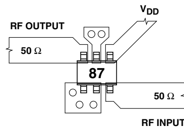
Figure 14. RF Layout.
