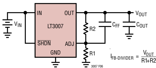
Figure 6. Feedforward Capacitor
