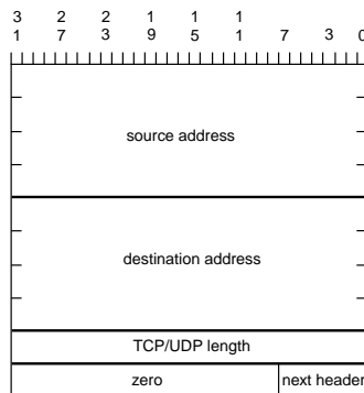
Figure 26-17. IPv6 Pseudo Header for Checksum Calculation
