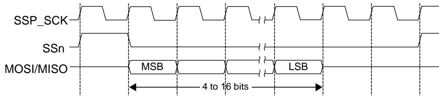
Figure 17-9. Texas Instruments Synchronous Serial Frame Format (Single Transfer)
