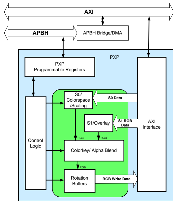
Figure 34-1. Pixel Pipeline (PXP) Block Diagram
