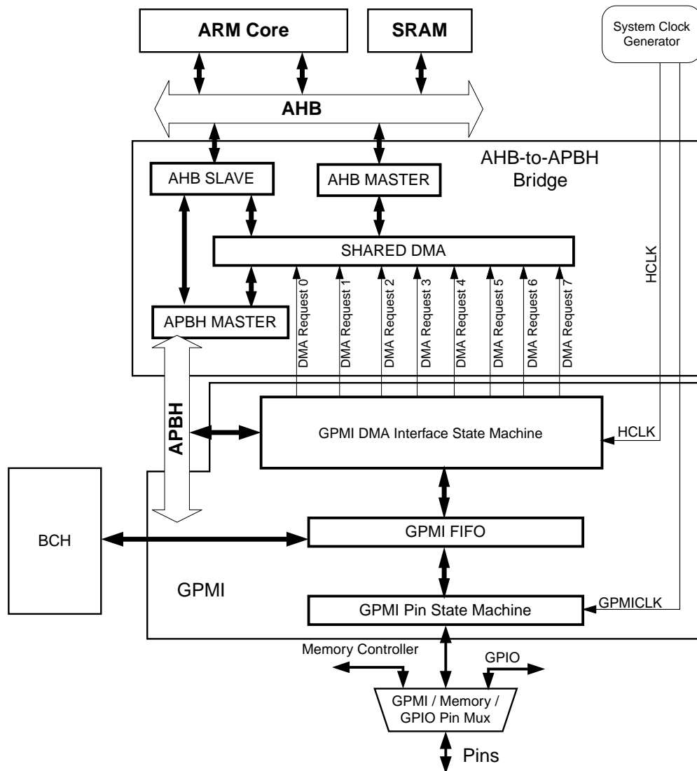
Figure 15-1. General-Purpose Media Interface Controller Block Diagram
