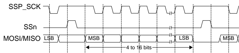
Figure 17-6. Motorola SPI Frame Format (Continuous Transfer) with POLARITY=1 and PHASE=0
