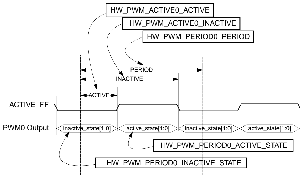
Figure 28-2. PWM Output Example
