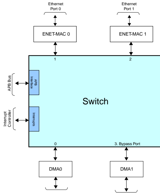
Figure 29-2. Switch Interface
