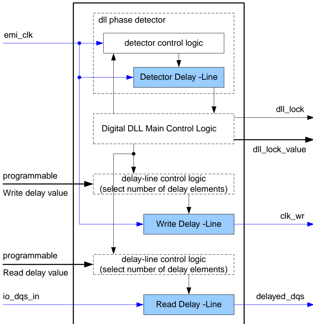
Figure 14-13. Digital DLL
