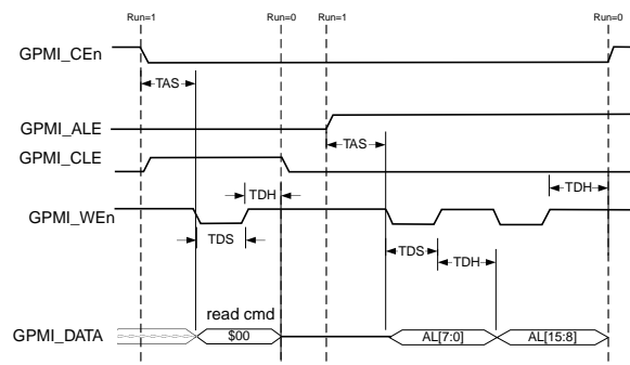
Figure 15-4. NAND Command and Address Timing Example
