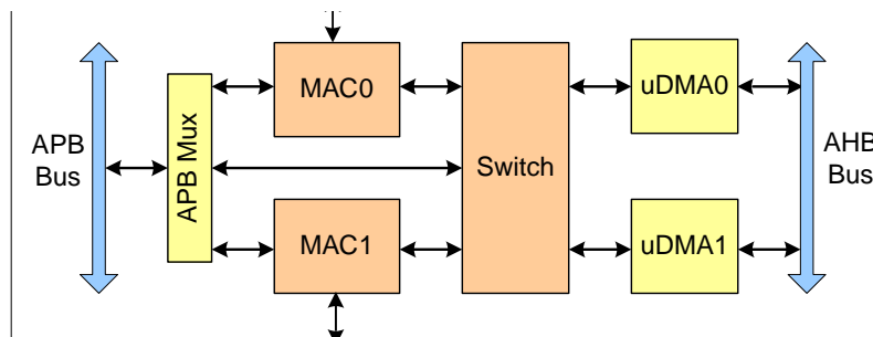
Figure 26-1. ENET Overview Block Diagram
