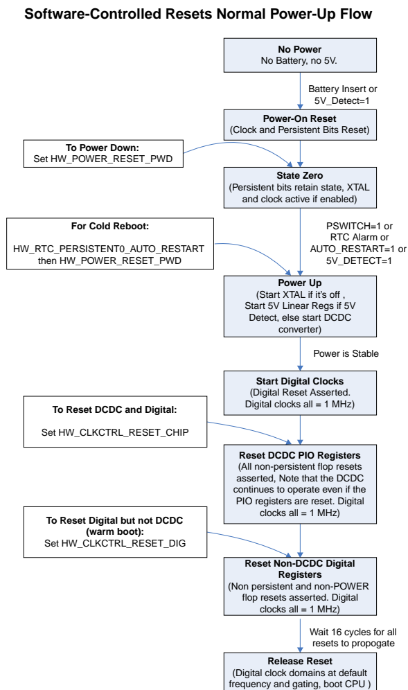
Figure 11-3. Power-Up, Power-Down, and Reset Flow Chart
