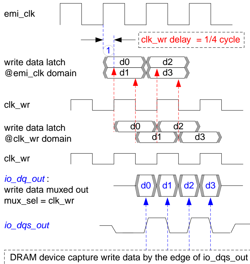
Figure 14-12. Write Data Path
