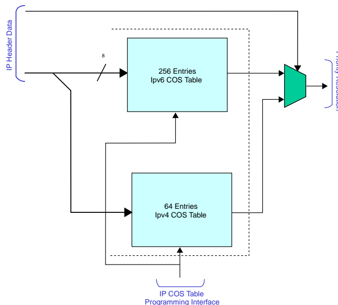
Figure 29-6. IP COS Tables Overview
