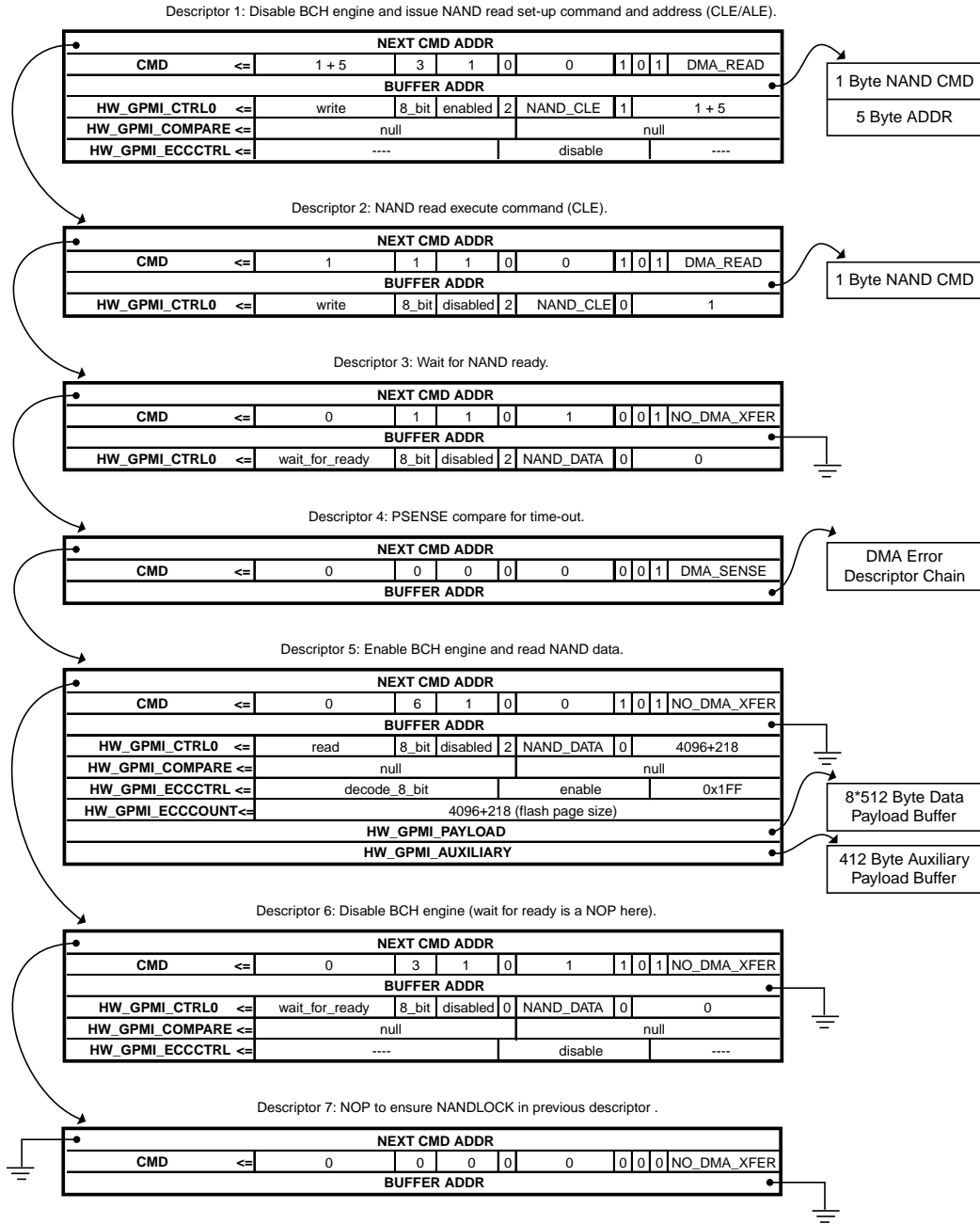
Figure 16-10. BCH Decode DMA Descriptor Chain
