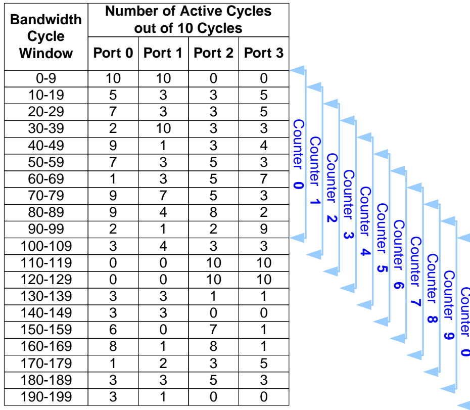
Figure 14-6. System Bandwidth Example
