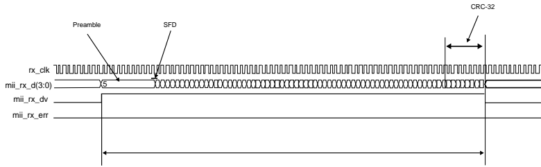
Figure 26-30. MII Receive Operation
