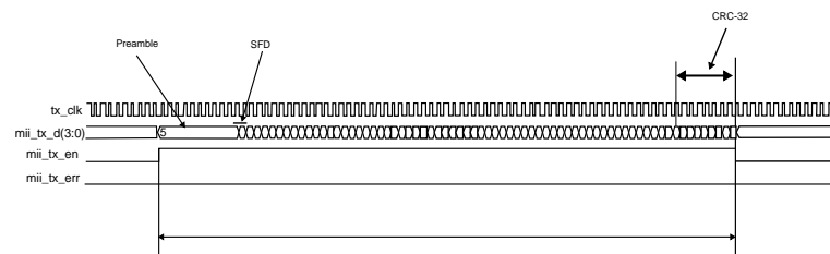
Figure 26-28. MII Transmit Operation - Errored Frame
