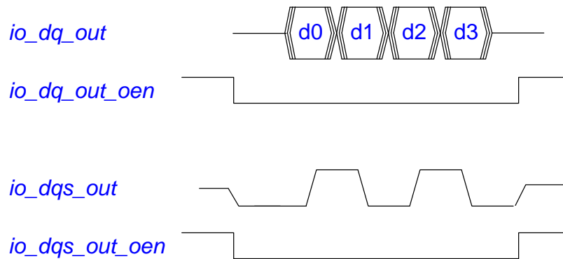
Figure 14-14. EMI I/O Output Enable
