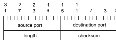
Figure 26-10. UDP Header Format
