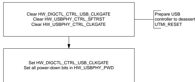
Figure 31-5. UTMI Powerdown
