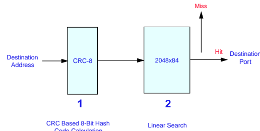
Figure 29-8. Port Look-Up Overview
