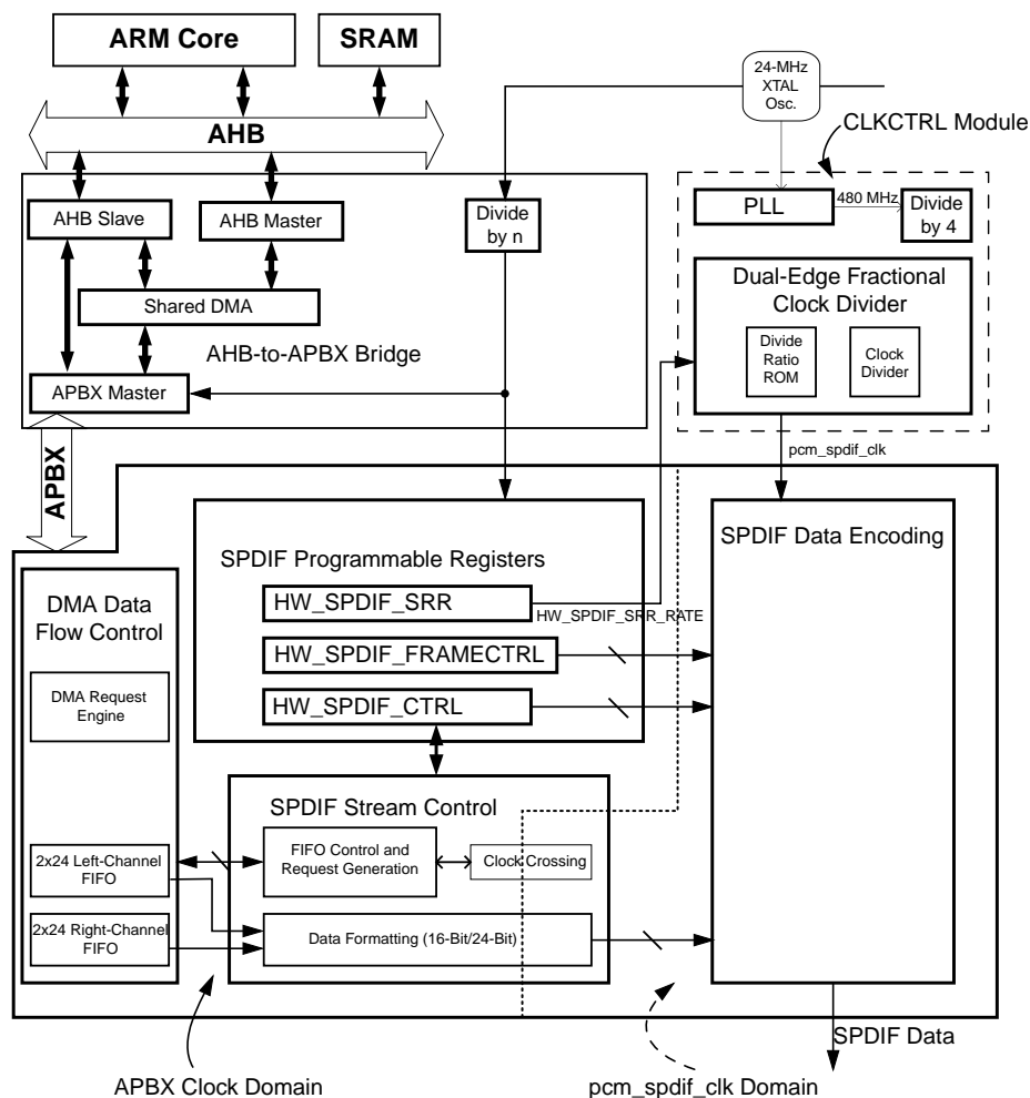
Figure 36-1. SPDIF Transmitter Block Diagram
