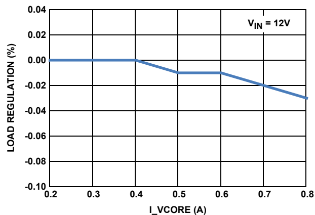
FIGURE 14. Vcore BUCK LOAD REGULATION
